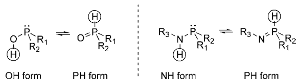
Figure 1. Phosphinous acid/SPO tautomerism (left) and aminophosphane/SIP tautomerism (right).
